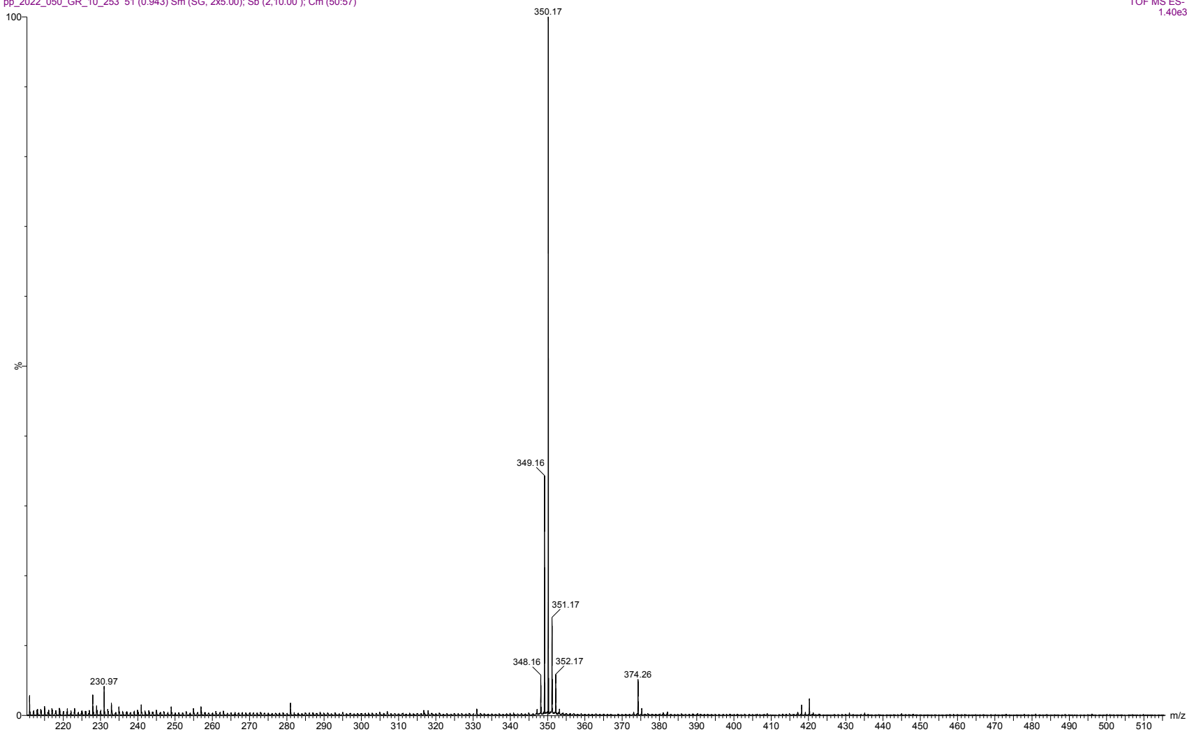
ESI-MS spectrum for sample GR-10-253. Shows monoisotopic [M-H]- mass.
